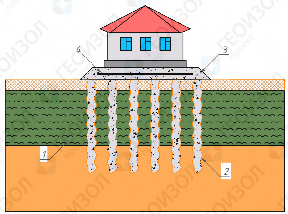
Sectional view
