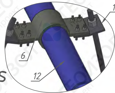
Fastening of pipes
