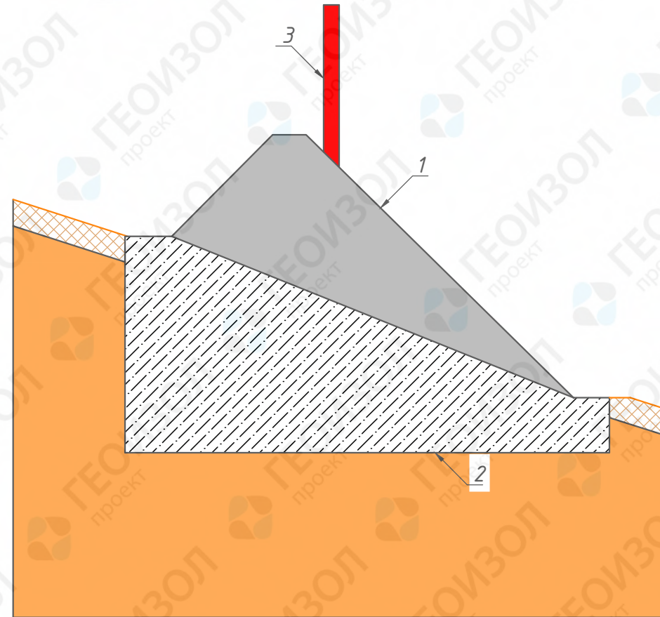
Sectional view
