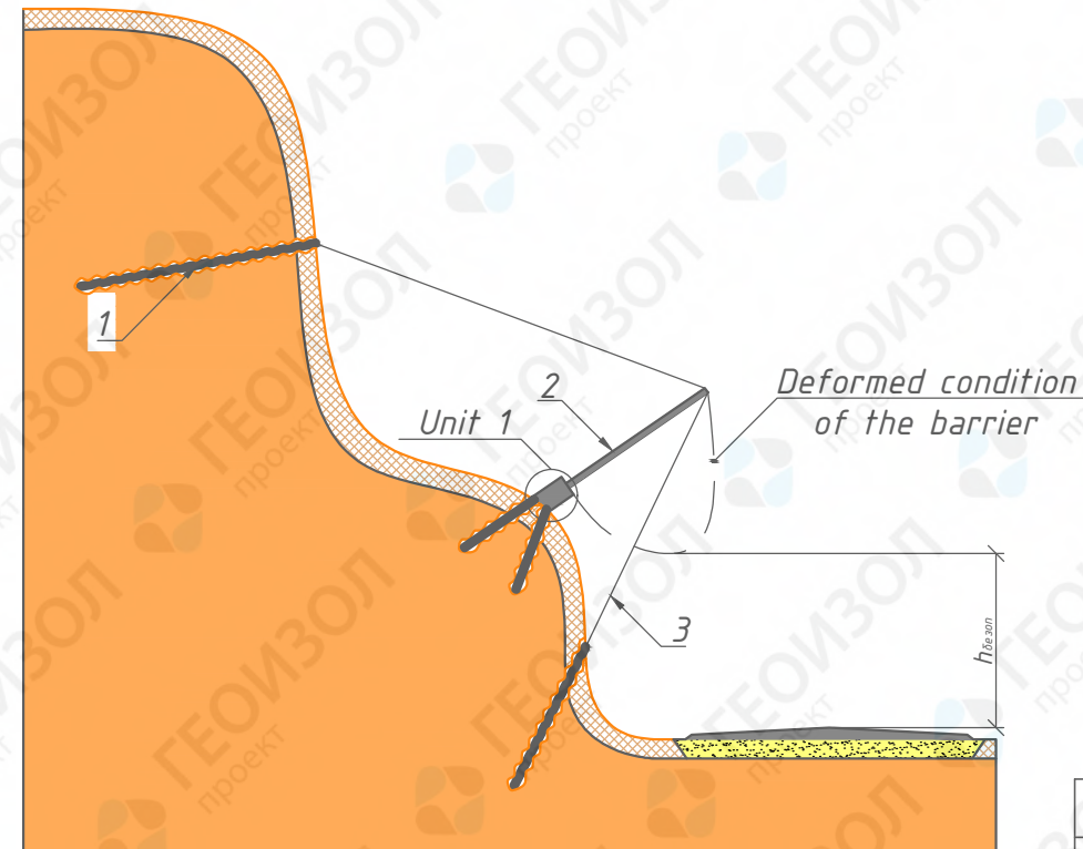
Sectional view
