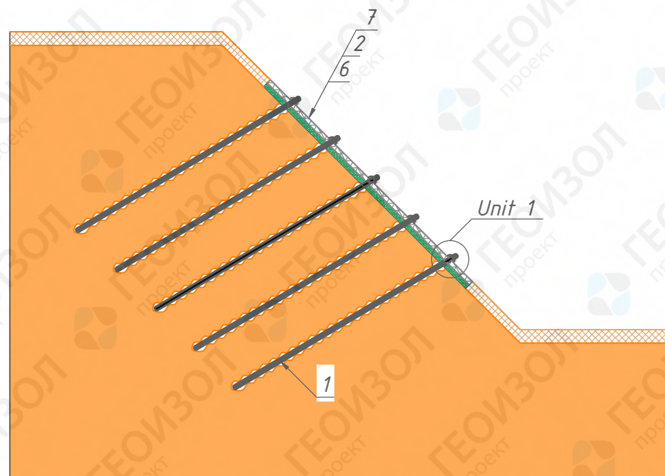
Sectional view
