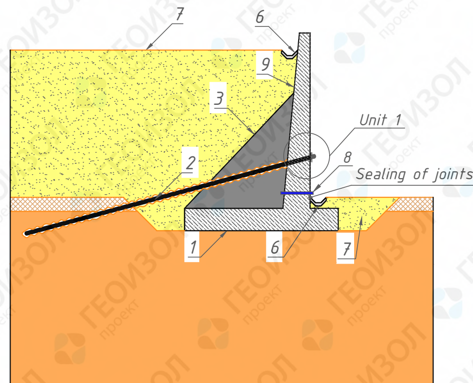
Sectional view
