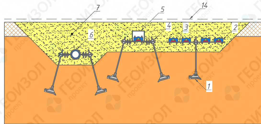
Fastening of pipes
