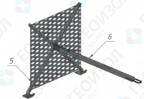
Snow umbrella
