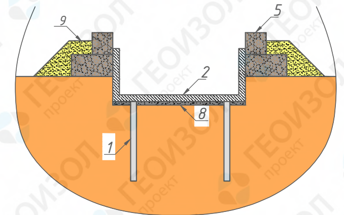
Sectional view of the debris flow channel
